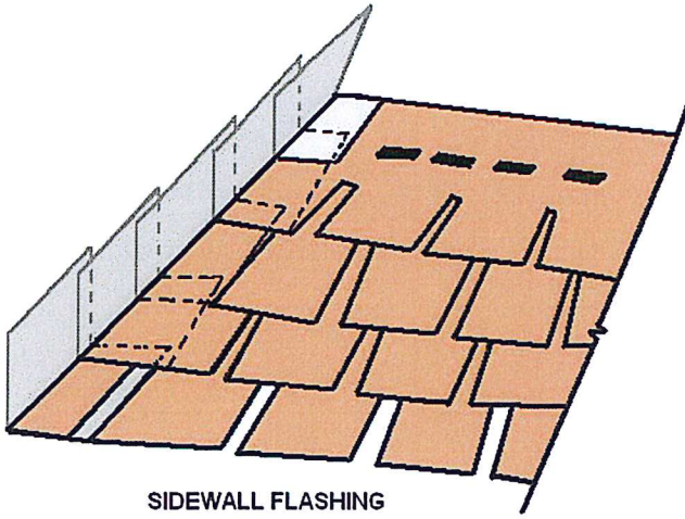
SIDEWALL FLASHING
